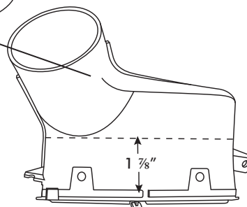
Bottom of Center Louver Assembly
