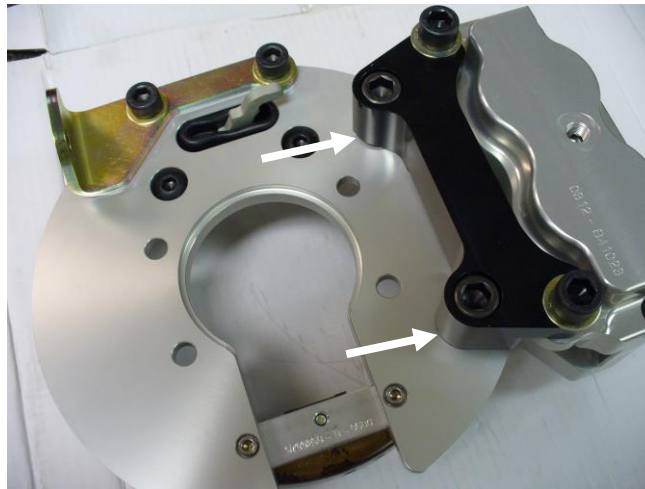
Figure 6: Shim locations
